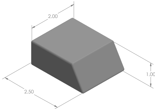
MODEL: SA242323 MAT'L: TUNGSTEN WEIGHT: 1.30kg DIMENSIONS: INCH
