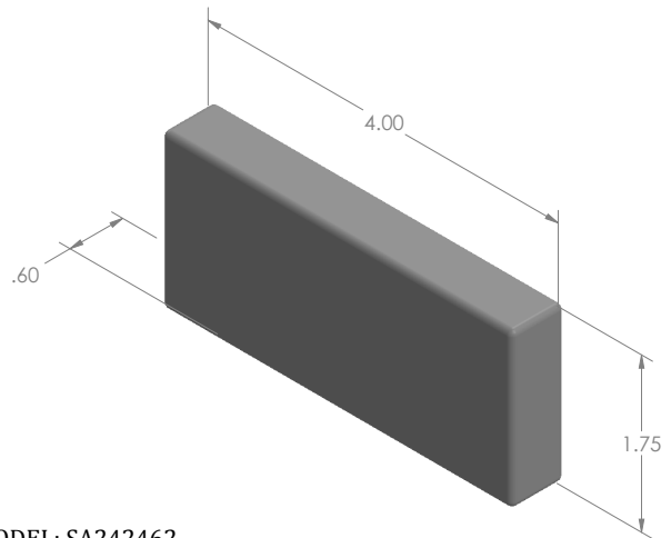
MODEL: SA242462 MAT'L: TUNGSTEN WEIGHT: 1.23kg DIMENSIONS: INCH
