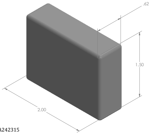
MODEL: SA242315 MAT'L: TUNGSTEN WEIGHT: 0.54kg DIMENSIONS: INCH
