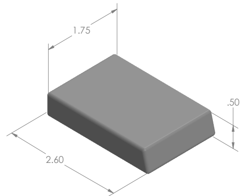
MODEL: SA242348 MAT'L: TUNGSTEN WEIGHT: 0.65kg DIMENSIONS: INCH
