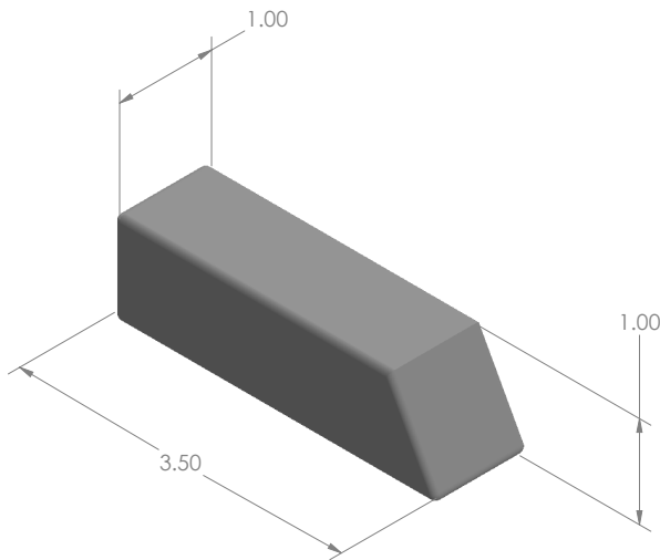
MODEL: SA242429 MAT'L: TUNGSTEN WEIGHT: 0.96kg DIMENSIONS: INCH
