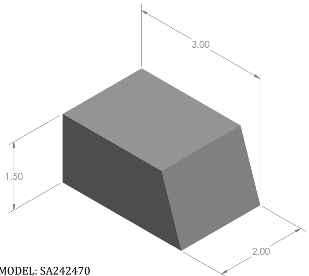
MODEL: SA242470 MAT'L: TUNGSTEN WEIGHT: 2.43kg DIMENSIONS: INCH
