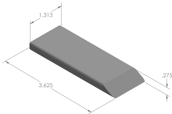
MODEL: SA242339 MAT'L: TUNGSTEN WEIGHT: 0.36kg DIMENSIONS: INCH
