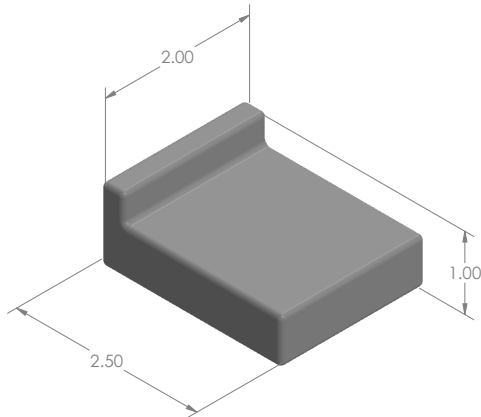
MODEL: SA242336 MAT'L: TUNGSTEN WEIGHT: 0.98kg DIMENSIONS: INCH
