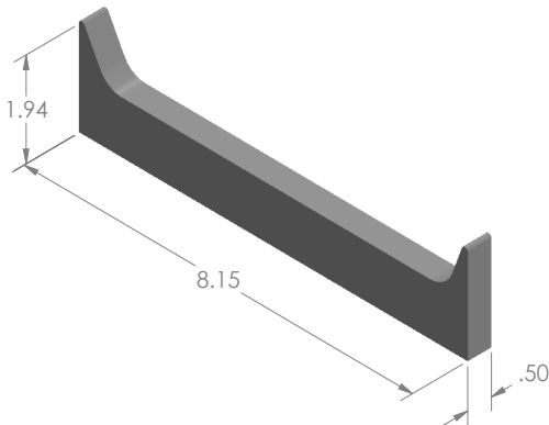
MODEL: SA242347 MAT'L: TUNGSTEN WEIGHT: 1.37kg DIMENSIONS: INCH
