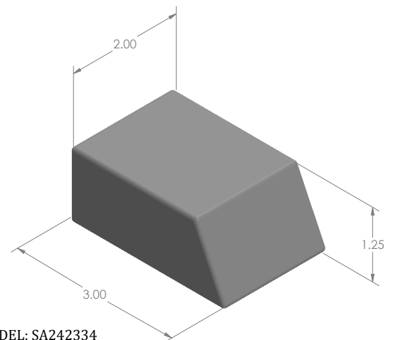
MODEL: SA242334 MAT'L: TUNGSTEN WEIGHT: 2.01kg DIMENSIONS: INCH
