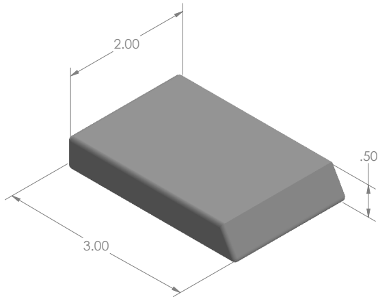
MODEL: SA242380 MAT'L: TUNGSTEN WEIGHT: 0.85kg DIMENSIONS: INCH
