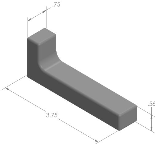
MODEL: SA242357 MAT'L: TUNGSTEN WEIGHT: 0.55kg DIMENSIONS: INCH
