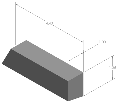
MODEL: SA242458 MAT'L: TUNGSTEN WEIGHT: 1.48kg DIMENSIONS: INCH
