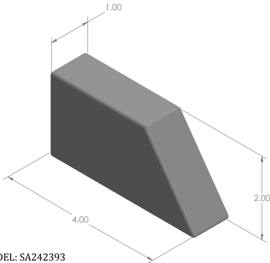
MODEL: SA242393 MAT'L: TUNGSTEN WEIGHT: 1.97kg DIMENSIONS: INCH
