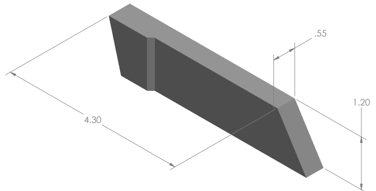
MODEL: SA242459 MAT'L: TUNGSTEN WEIGHT: 0.75kg DIMENSIONS: INCH
