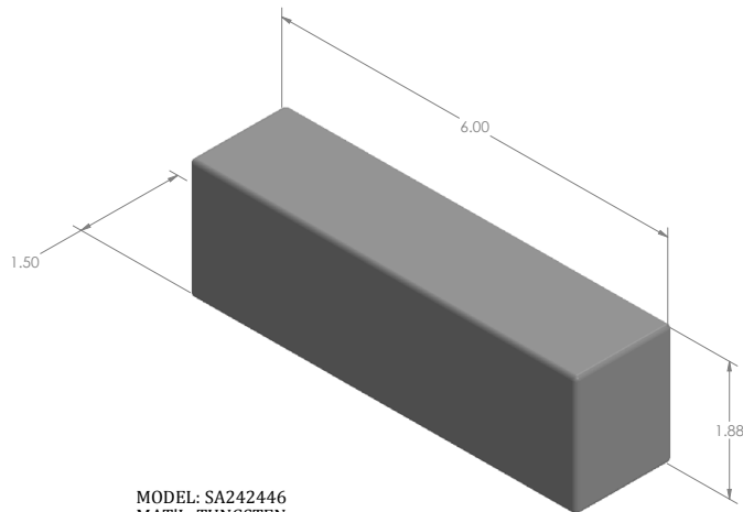
MODEL: SA242446 MAT'L: TUNGSTEN WEIGHT: 4.97kg DIMENSIONS: INCH
