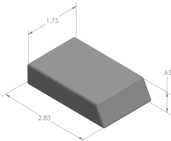
MODEL: SA242395 MAT'L: TUNGSTEN WEIGHT: 0.87kg DIMENSIONS: INCH
