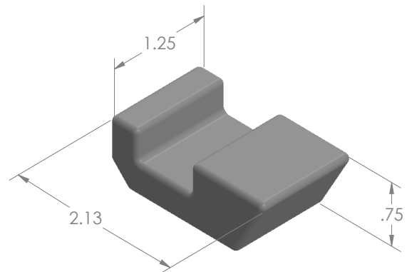
MODEL: SA242330 MAT'L: TUNGSTEN WEIGHT: 0.42kg DIMENSIONS: INCH
