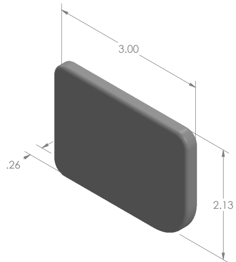
MODEL: SA242396 MAT'L: TUNGSTEN WEIGHT: 0.47kg DIMENSIONS: INCH
