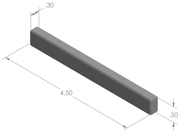
MODEL: SA242376 MAT'L: TUNGSTEN WEIGHT: 0.19kg DIMENSIONS: INCH
