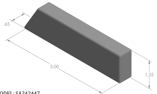
MODEL: SA242447 MAT'L: TUNGSTEN WEIGHT: 1.11kg DIMENSIONS: INCH
