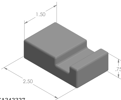
MODEL: SA242327 MAT'L: TUNGSTEN WEIGHT: 0.74kg DIMENSIONS: INCH
