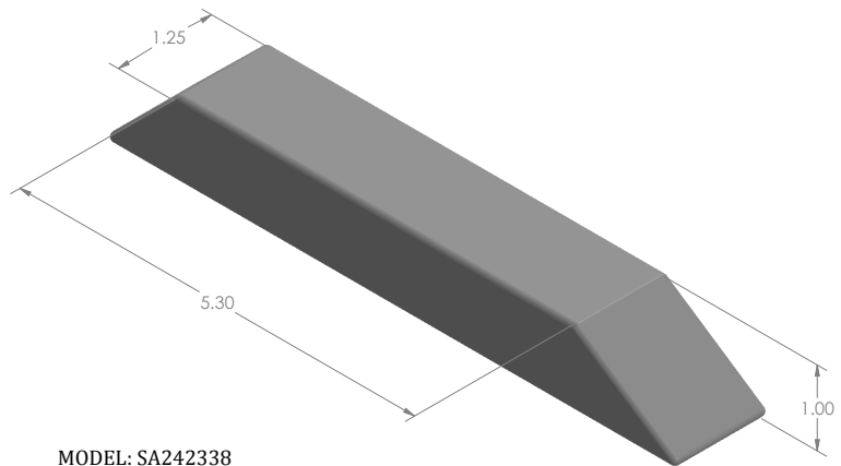
MODEL: SA242338 MAT'L: TUNGSTEN WEIGHT: 2.42kg DIMENSIONS: INCH
