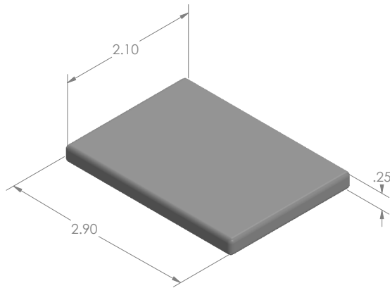
MODEL: SA242349 MAT'L: TUNGSTEN WEIGHT: 0.44kg DIMENSIONS: INCH
