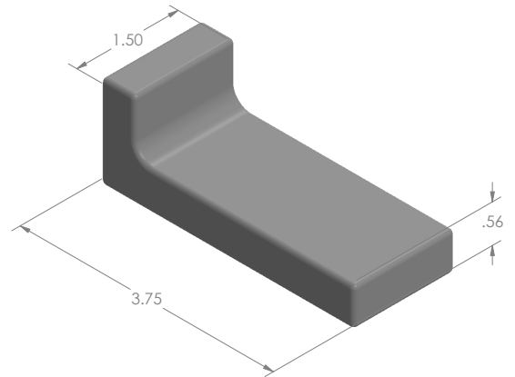
MODEL: SA242136 MAT'L: TUNGSTEN WEIGHT: 1.24kg DIMENSIONS: INCH
