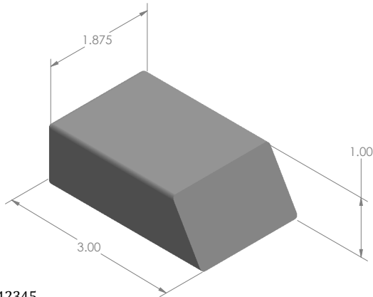
MODEL: SA242345 MAT'L: TUNGSTEN WEIGHT: 1.49kg DIMENSIONS: INCH
