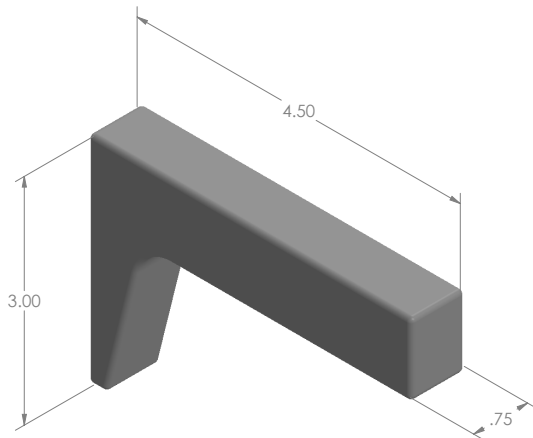
MODEL: SA242329 MAT'L: TUNGSTEN WEIGHT: 1.21kg DIMENSIONS: INCH
