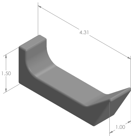
MODEL: SA242364 MAT'L: TUNGSTEN WEIGHT: 0.91kg DIMENSIONS: INCH
