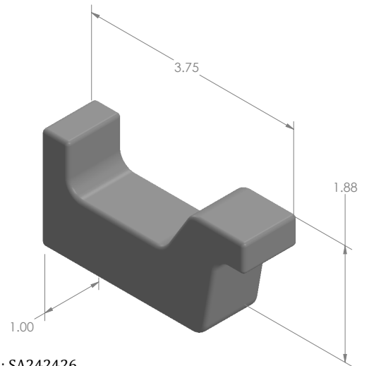
MODEL: SA242426 MAT'L: TUNGSTEN WEIGHT: 1.34kg DIMENSIONS: INCH
