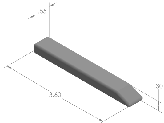
MODEL: SA242379 MAT'L: TUNGSTEN WEIGHT: 0.16kg DIMENSIONS: INCH
