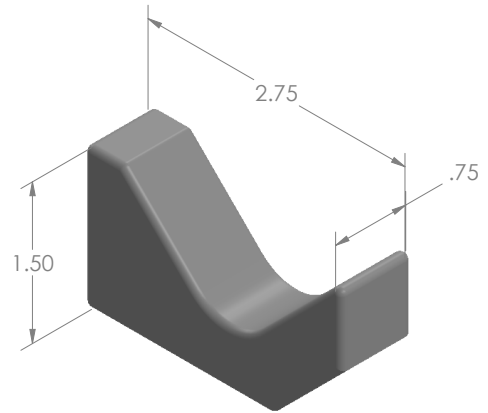
MODEL: SA242362 MAT'L: TUNGSTEN WEIGHT: 0.58kg DIMENSIONS: INCH
