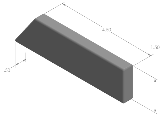
MODEL: SA242445 MAT'L: TUNGSTEN WEIGHT: 1.10kg DIMENSIONS: INCH
