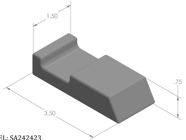
MODEL: SA242423 MAT'L: TUNGSTEN WEIGHT: 0.95kg DIMENSIONS: INCH
