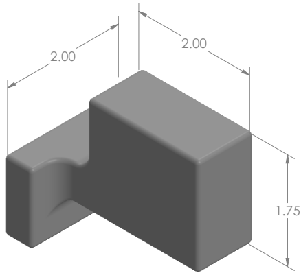
MODEL: SA242422 MAT'L: TUNGSTEN WEIGHT: 1.50kg DIMENSIONS: INCH
